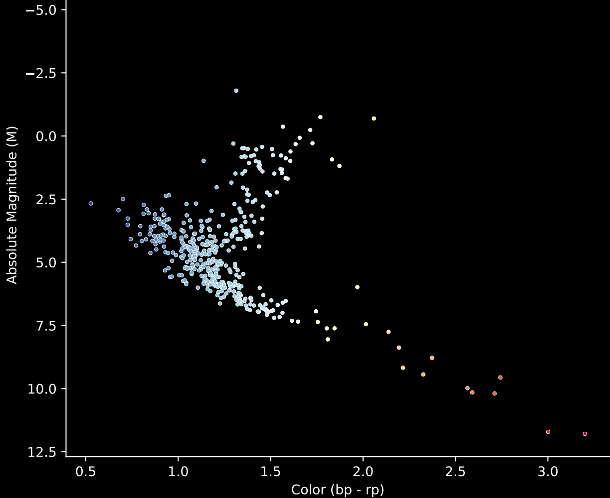
GALAH DR4 Field [6595] Stars (n= 441) Hertzsprung-Russel Diagram
