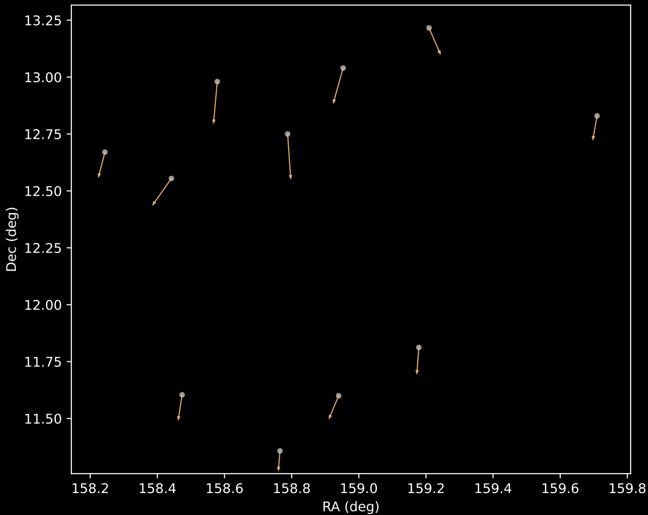
GALAH DR4 Cluster 23 Proper Motion Vectors (n=11)
