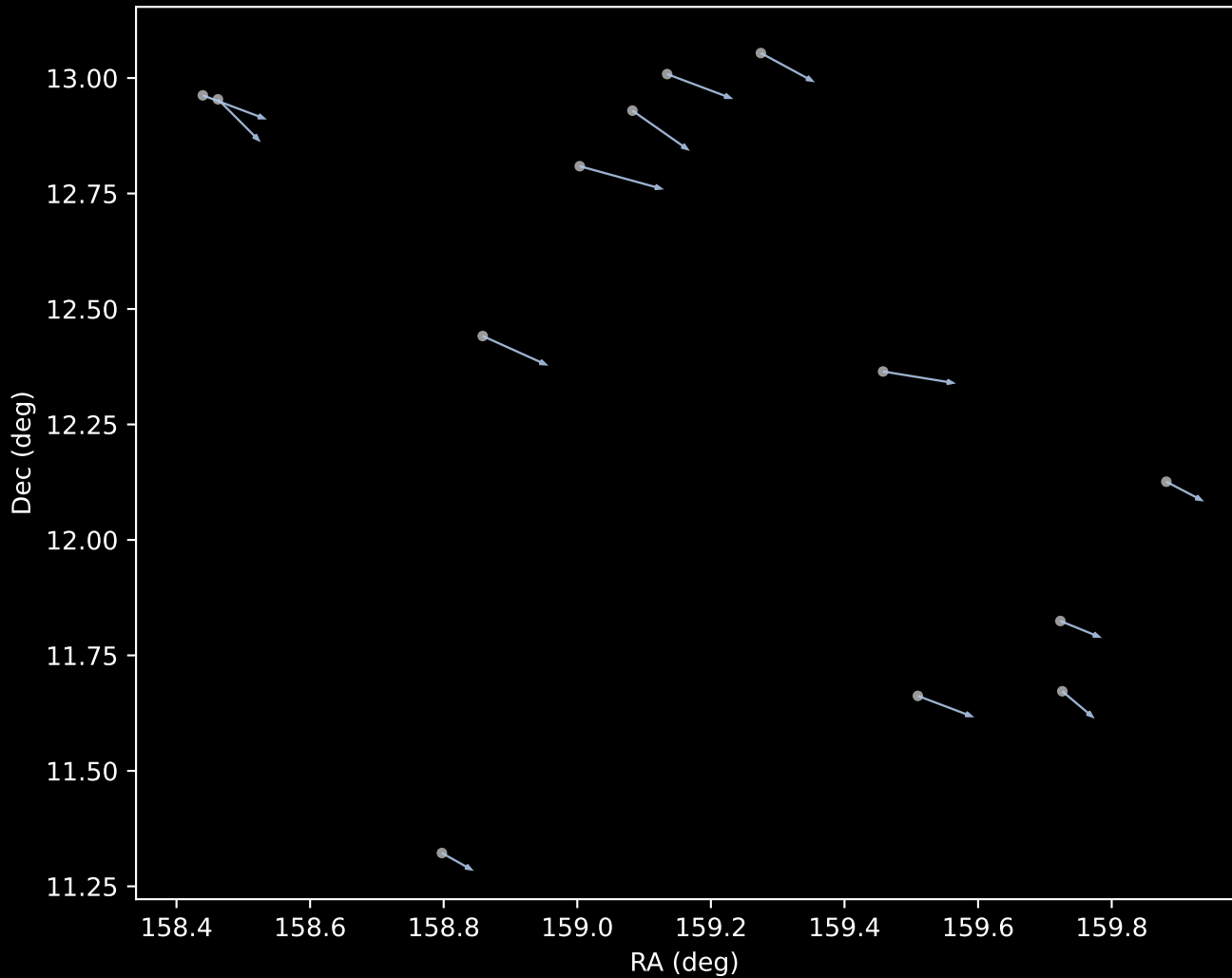
GALAH DR4 Cluster 21 Proper Motion Vectors (n=13)
