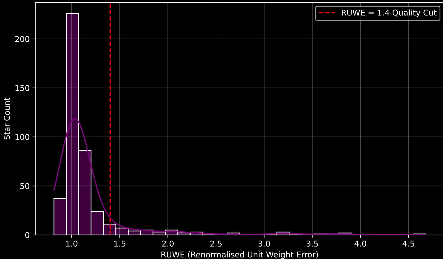
GALAH DR4 Field [6595] RUWE Distribution (n= 426)
