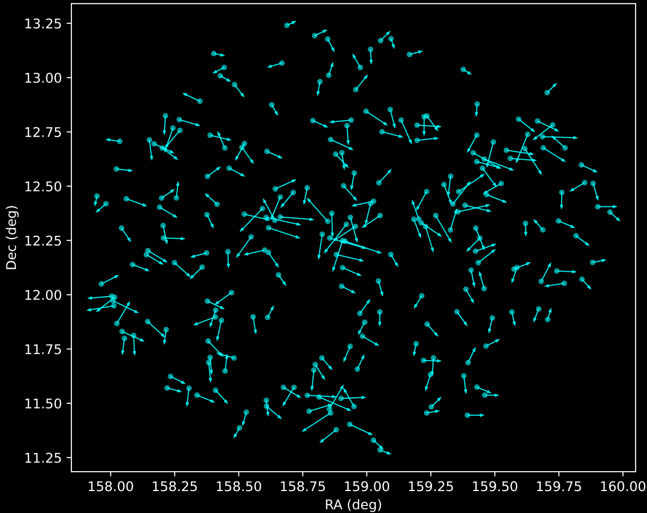
GALAH DR4 Noise Stream Proper Motion Vectors (n=231)
