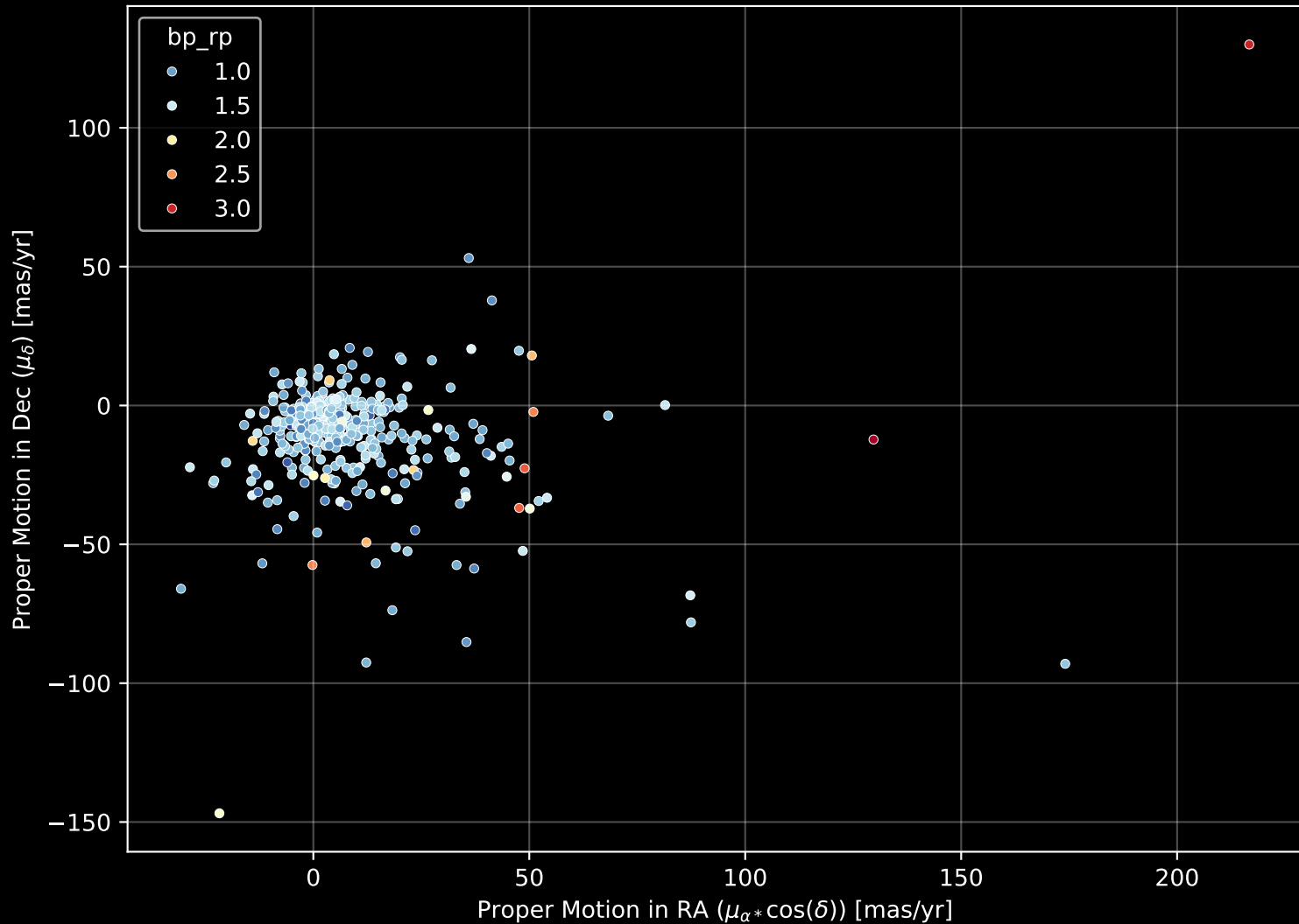
GALAH DR4 Field: [6595] Proper Motion Diagram (n= 441)
